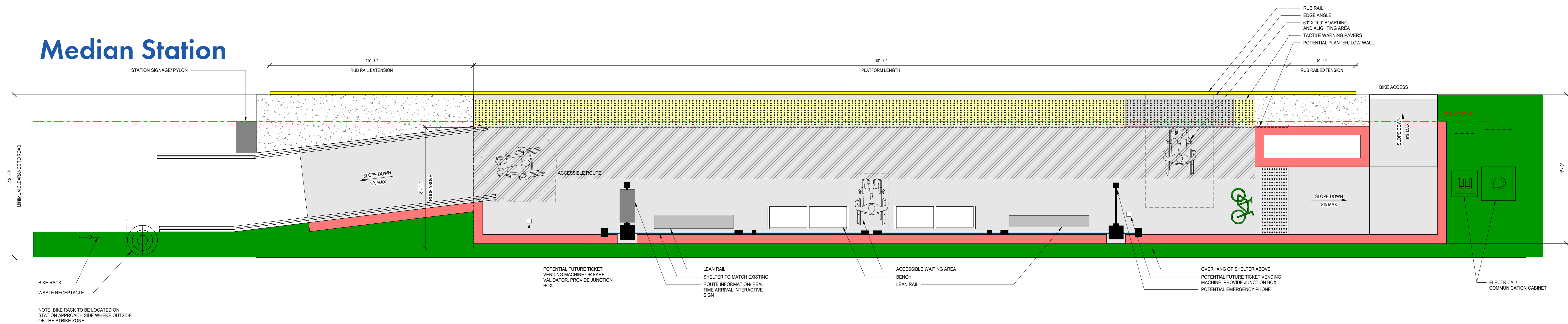
2 TYPICAL STATION PLAN- MEDIAN SCALE: 3/8" = 1'-0"
